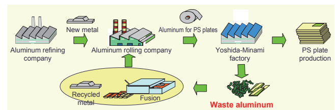
Figure 3 Closed loop recycling of cutting waste
