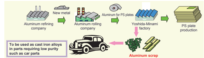
Figure 4 Conventional cutting waste recycling (cascade recycling)
